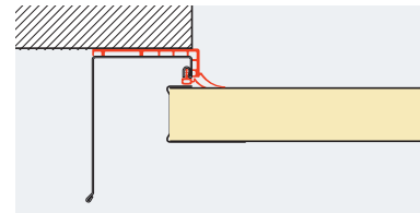
Side sealing
