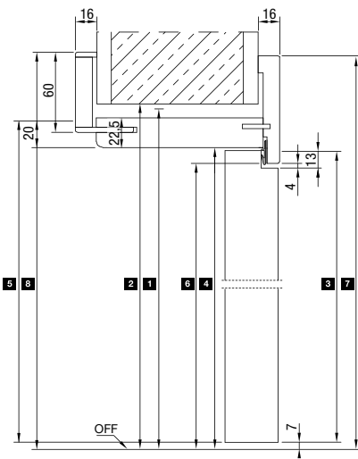
Vertical view
