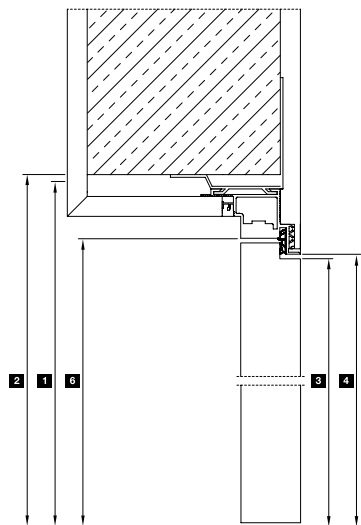
Vertical view with reverse-opening door leaf
