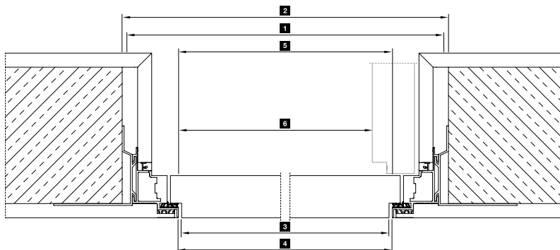
Horizontal view with reverse-opening door leaf
