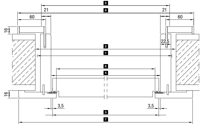
Horizontal views
