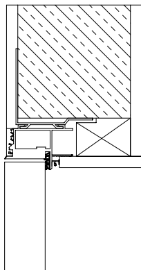
Horizontal sectional view with flush-closing door
