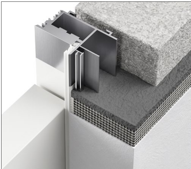
Additional use of a flexible woven fabric prevents cracks from forming in the plaster.
