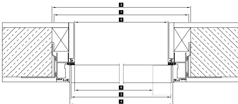
Horizontal view with flush door leaf
