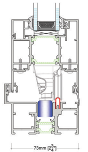
Standard threshold detail
