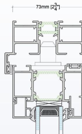
Head detail
